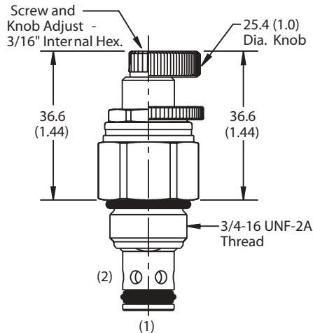
Screw/Knob Version
