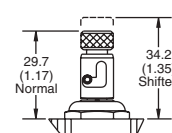
Push and Twist M.O. (Normally Closed Valves Only)
