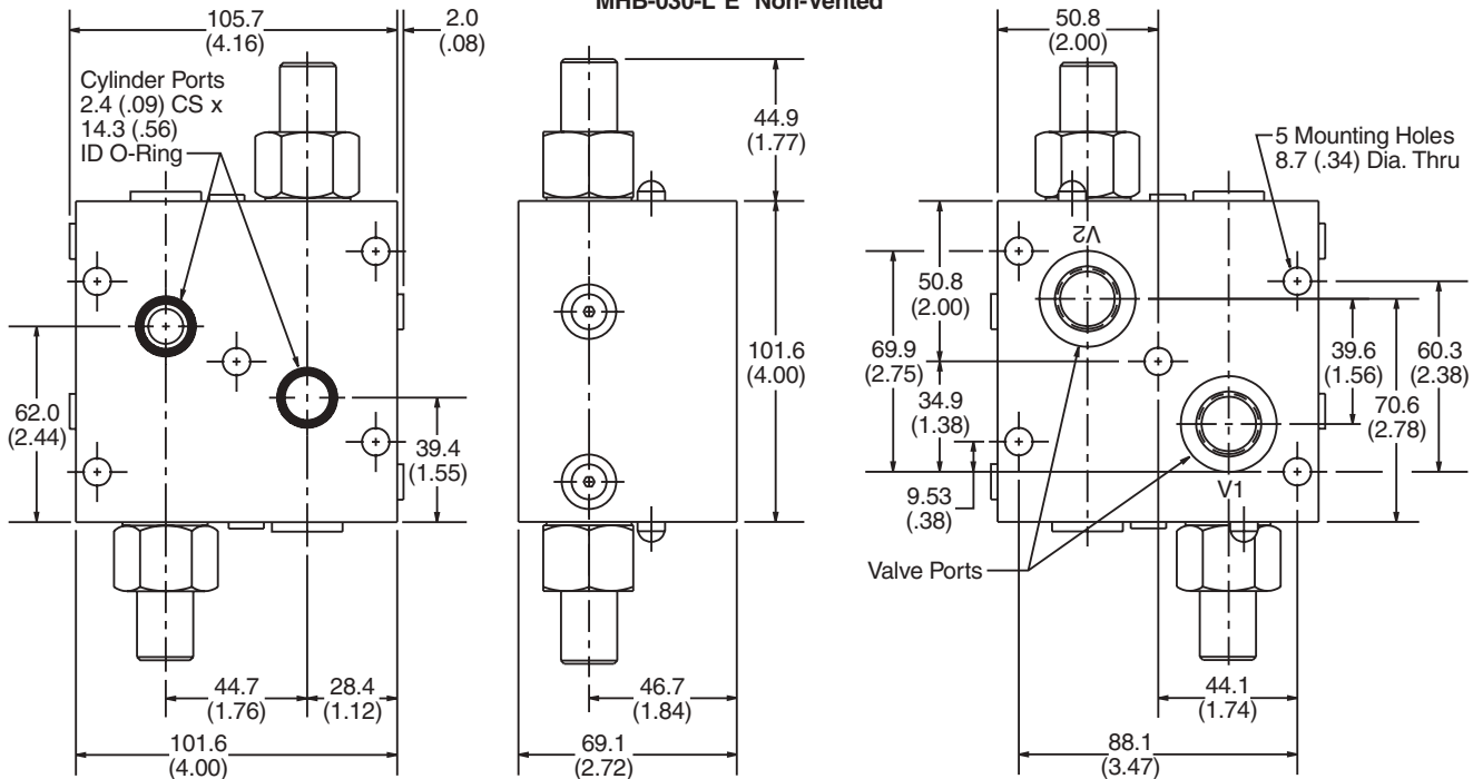
MHB-030-L*E* Non-Vented
