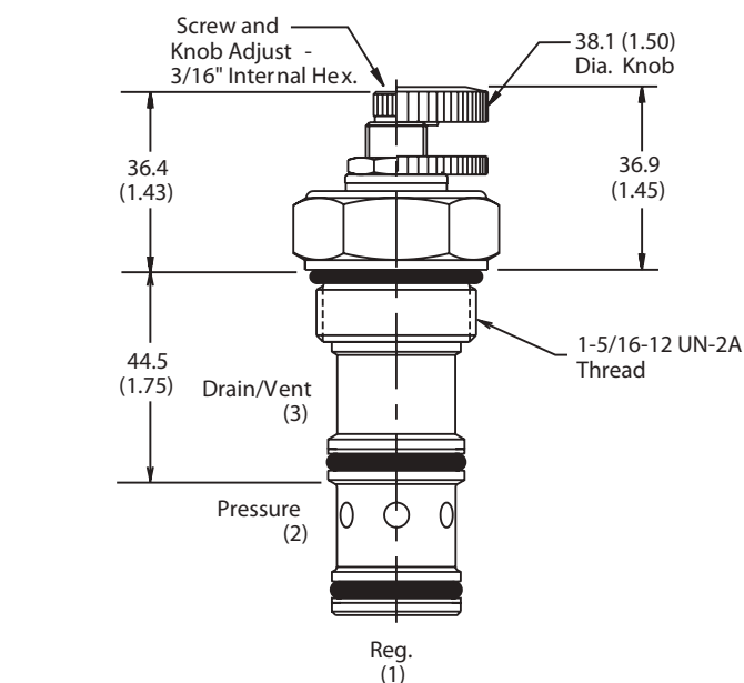
Screw/Knob Version
