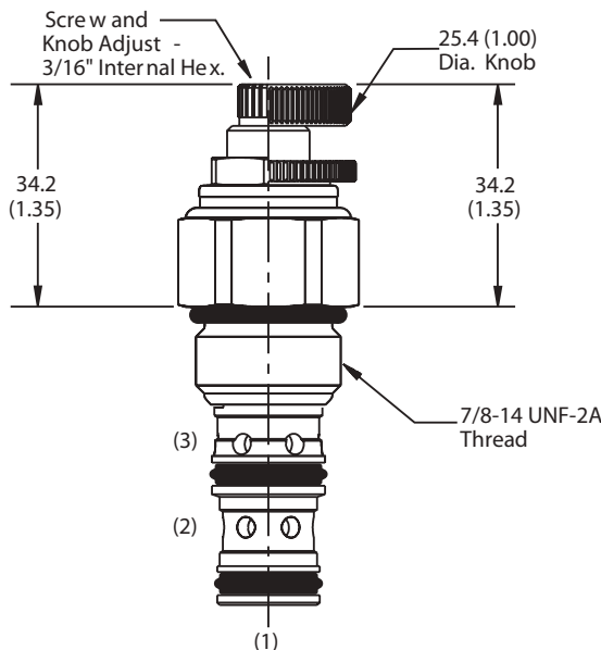
Screw/Knob Version
