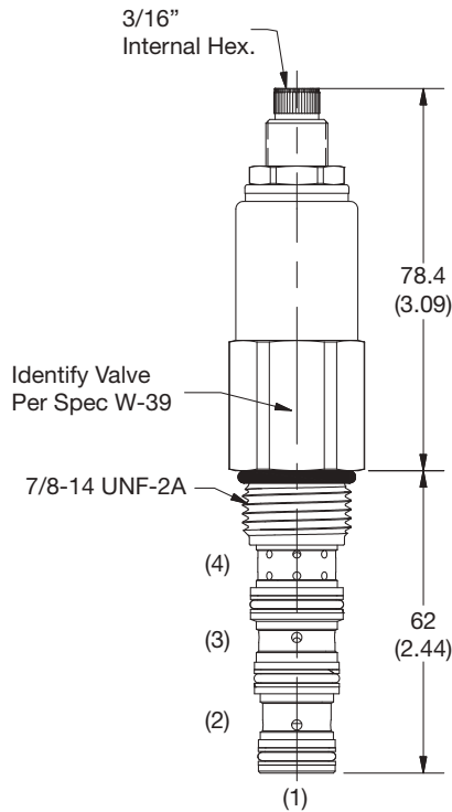
SCREW VERSION
