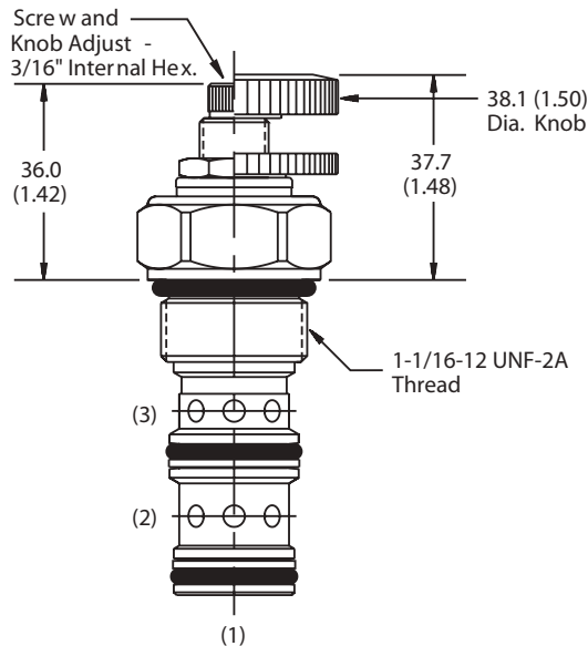
Screw/Knob Version
